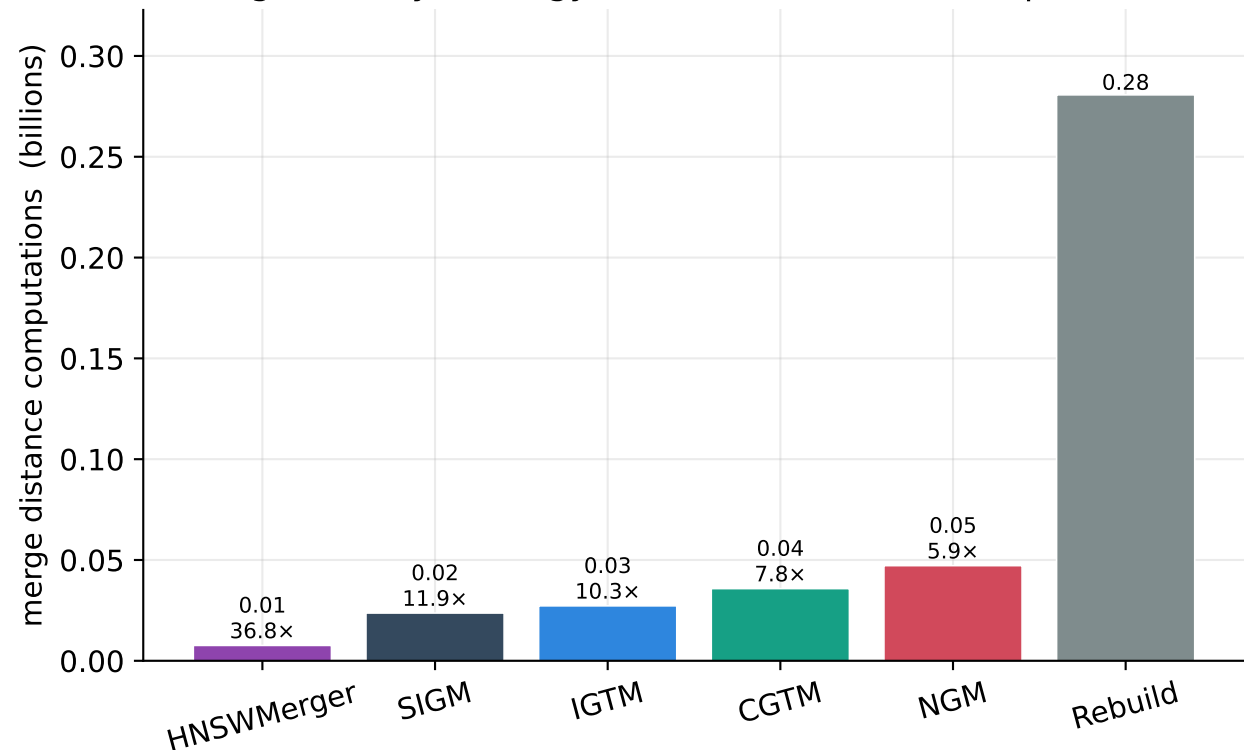
Merge cost by strategy (SIFT 100K (BIGANN), 2 partitions)
