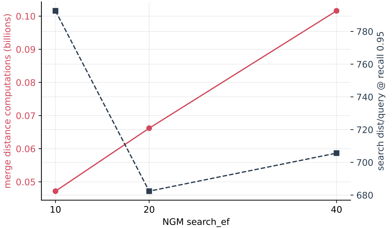
NGM: cost and search quality vs search_ef ([792.5877314606739, 682.3813236263719, 705.6337760831886])
