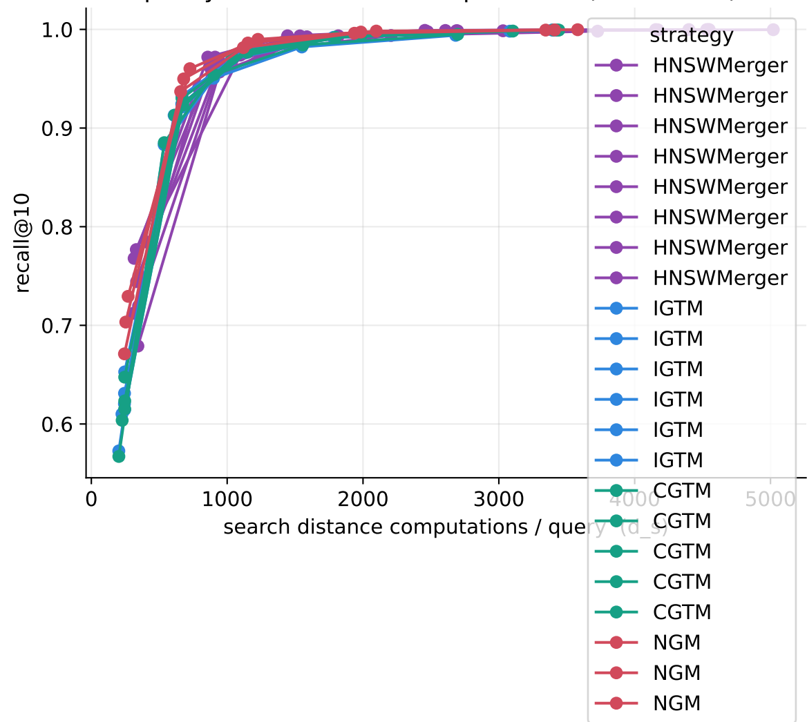
Search quality vs search cost at 2 partitions (SIFT 100K (BIGANN))
