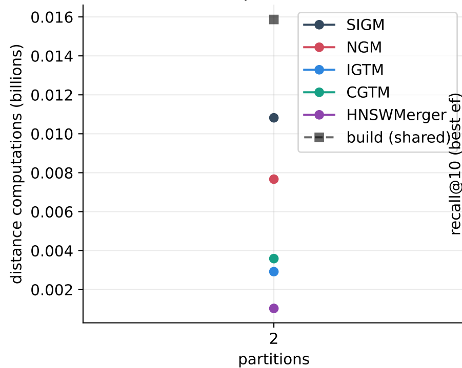
Cost vs partition count
