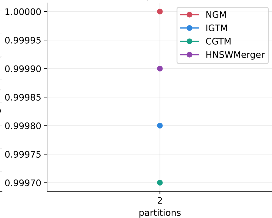
Recall vs partition count
