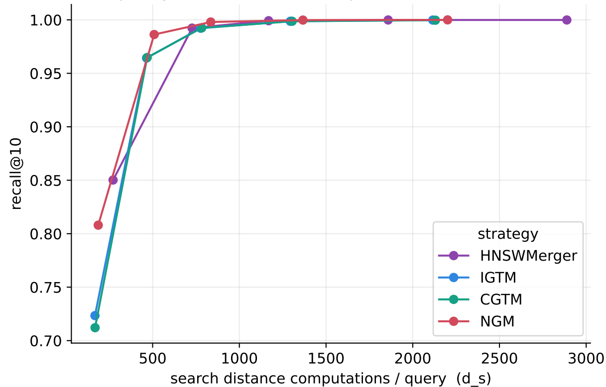
Search quality vs search cost at 2 partitions (SIFT 10K (BIGANN))
