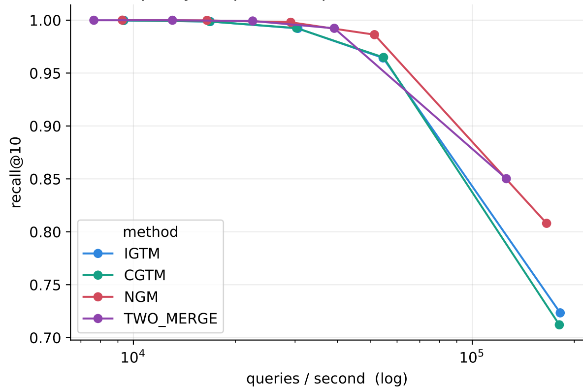
Search quality vs speed at 2 partitions (SIFT 10K (BIGANN))
