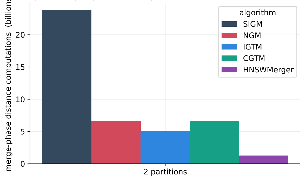
Merge cost by algorithm and partition count (SIFT 10M (BIGANN))
