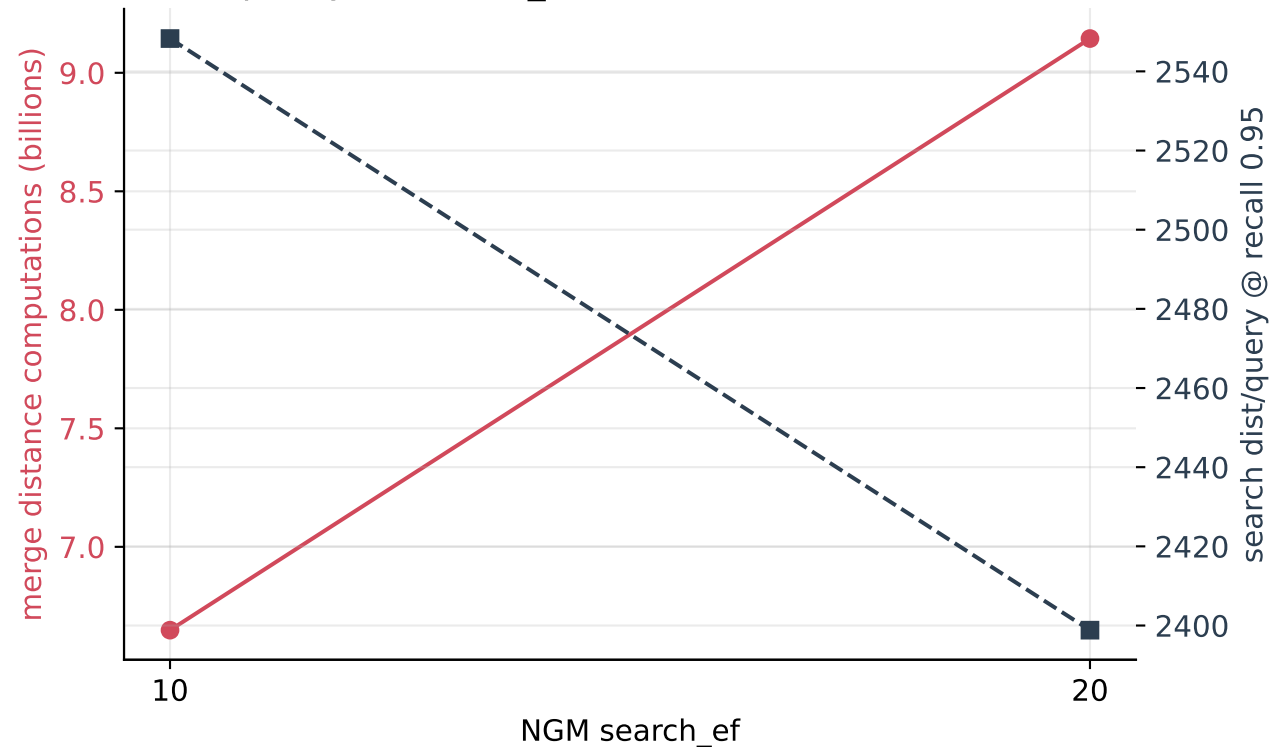
NGM: cost and search quality vs search_ef ([2548.2908514970045, 2398.827793706292])
