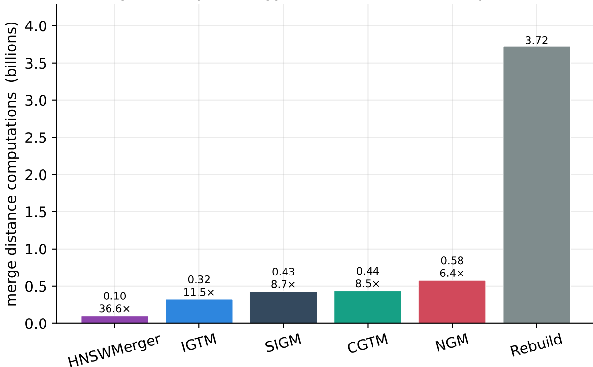
Merge cost by strategy (SIFT 1M (BIGANN), 2 partitions)
