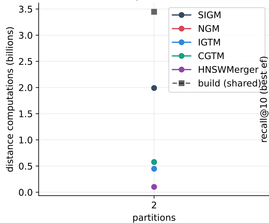
Cost vs partition count
