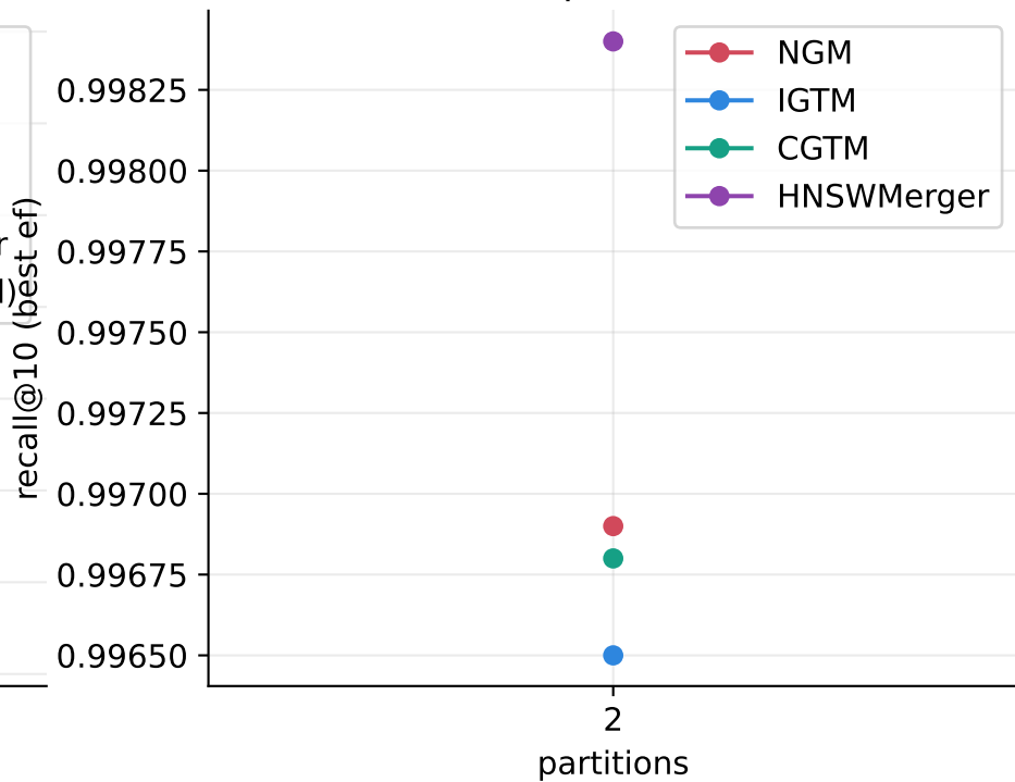
Recall vs partition count
