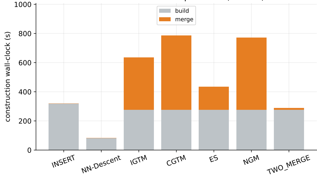
Construction time at 2 partitions (GIST1M)
