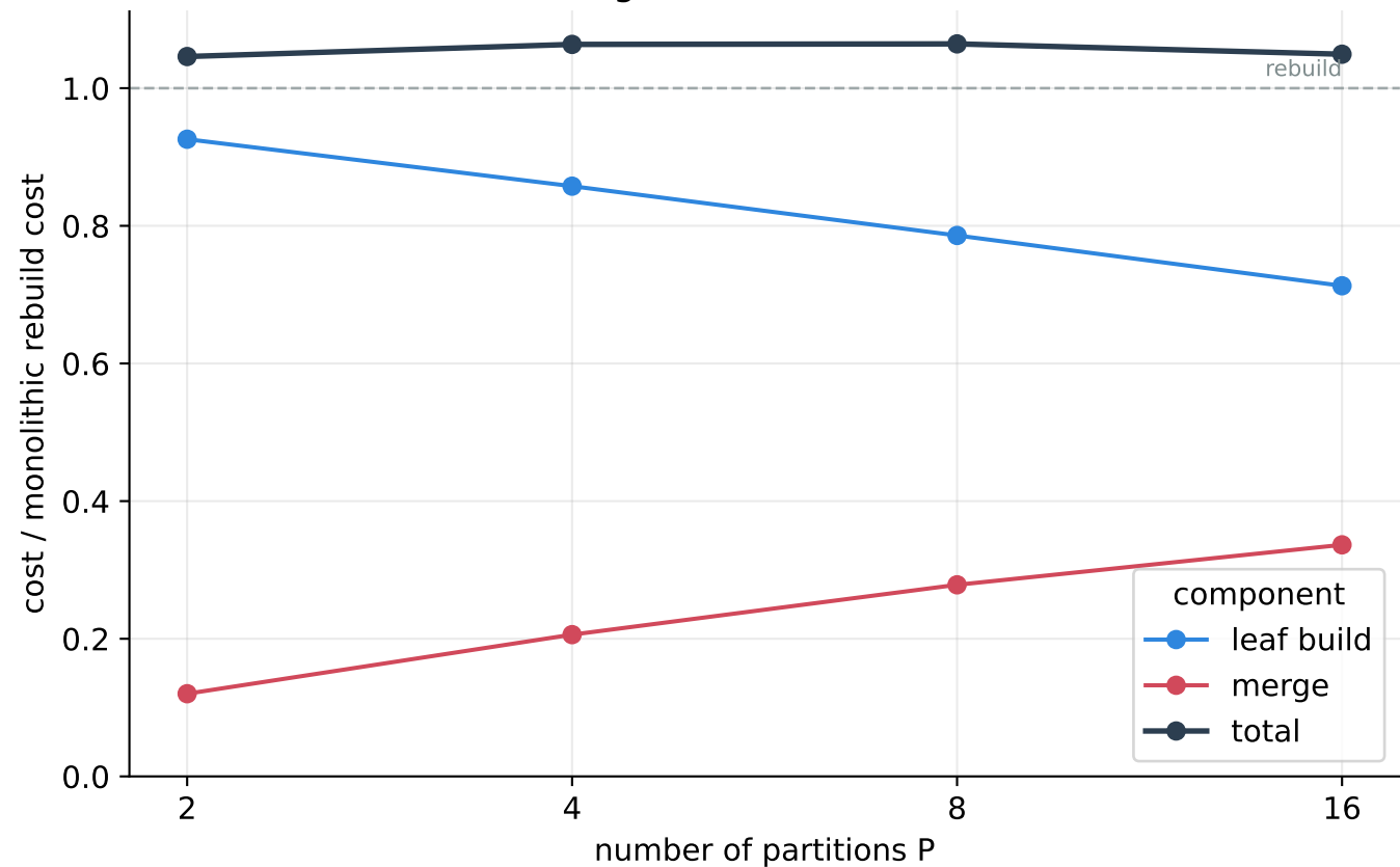
IGTM: build/merge/total vs P (SIFT 1M (BIGANN))
