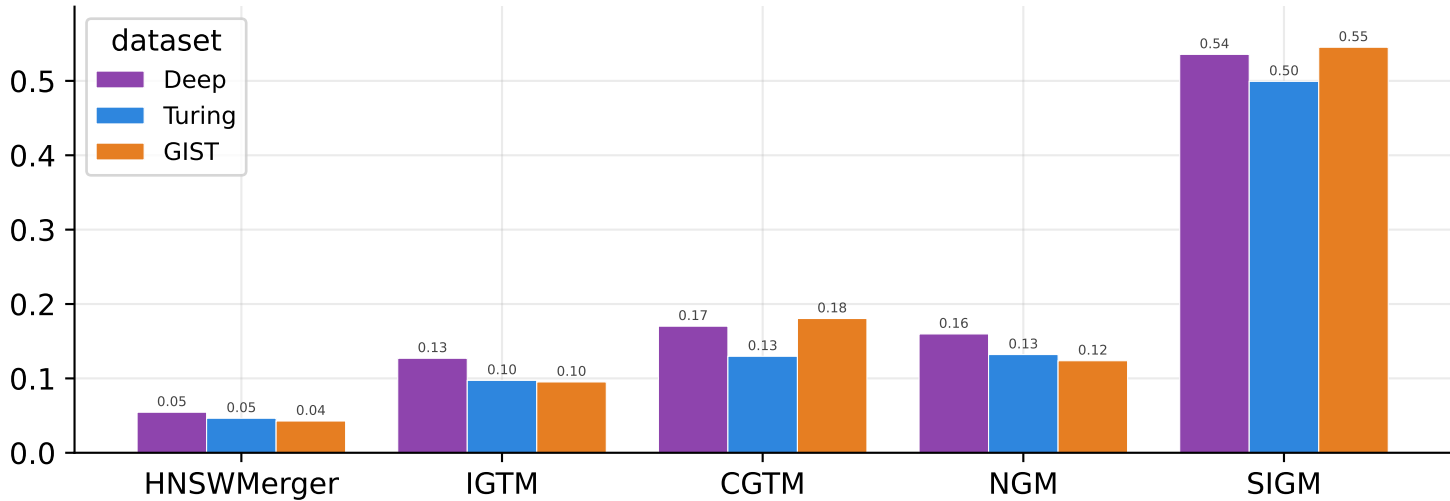
Strategy cost relative to full rebuild across datasets (1M)
