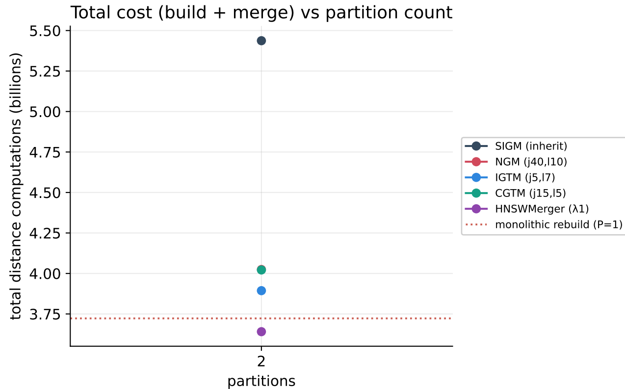
Total construction cost by strategy vs partition count (SIFT 1M (BIGANN))
