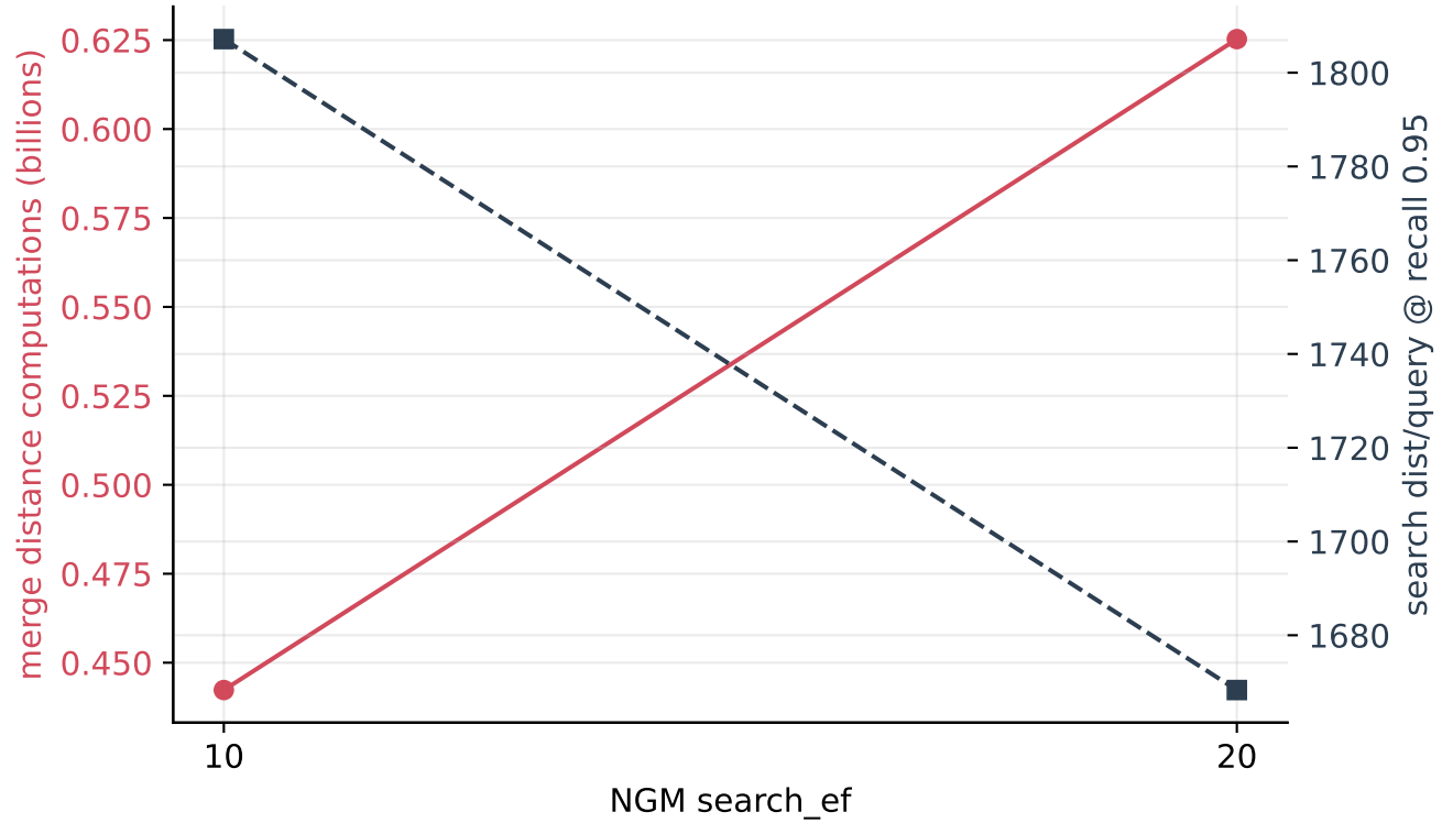
NGM: cost and search quality vs search_ef ([1807.1629230107496, 1668.3102829457357])
