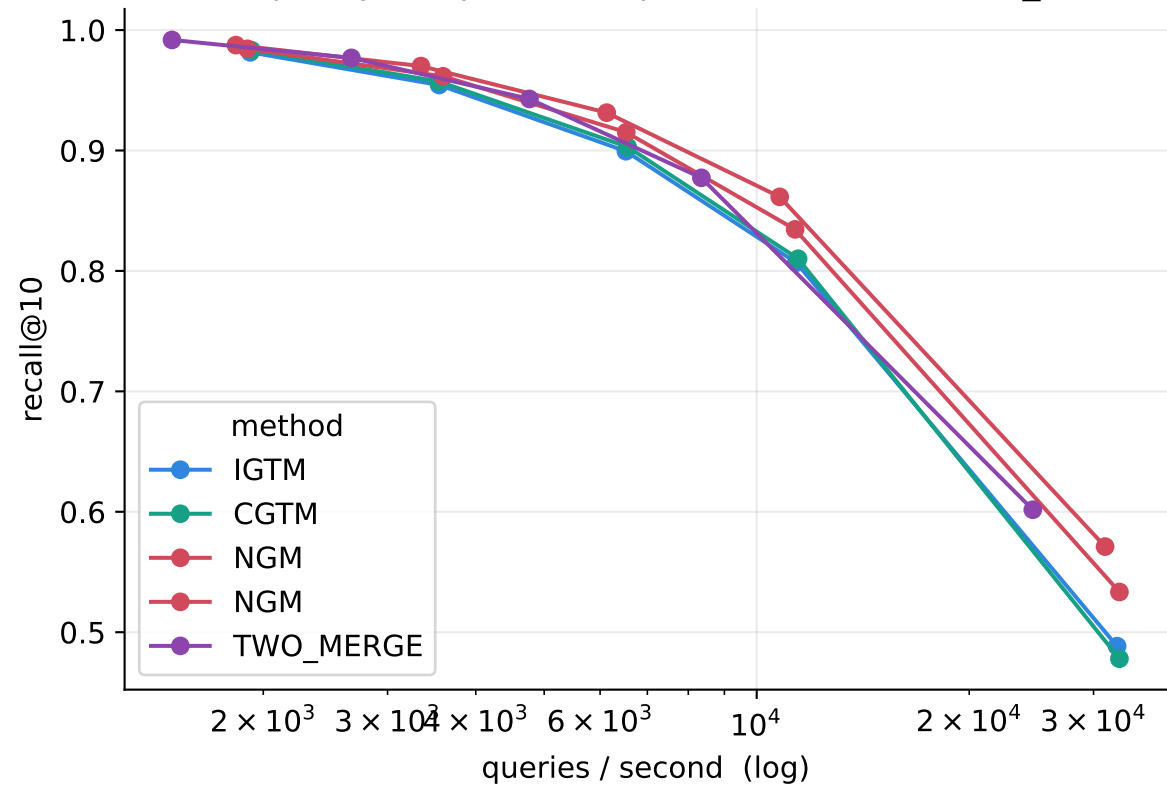
Search quality vs speed at 2 partitions (BIGANN1M_32EFC)
