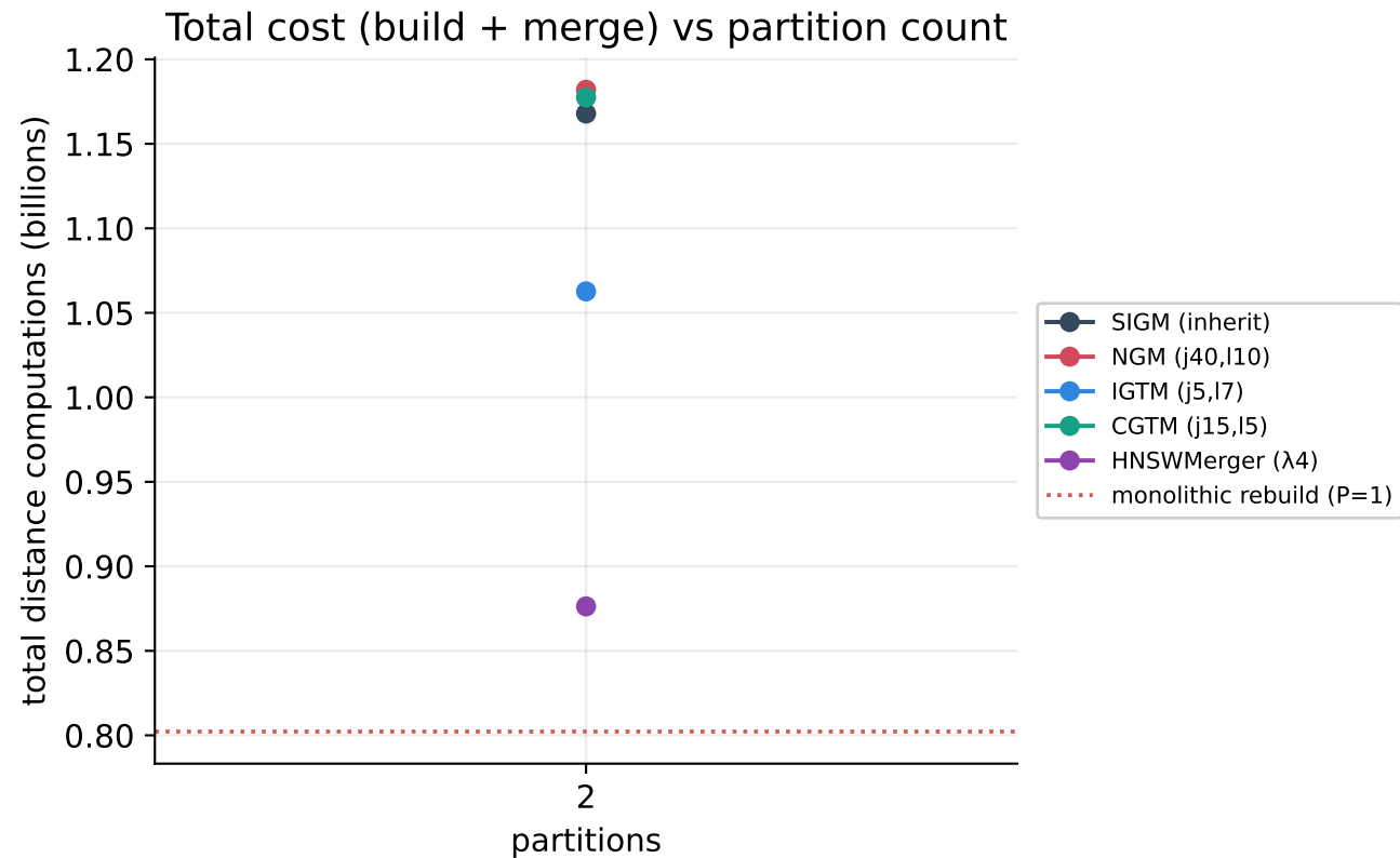
Total construction cost by strategy vs partition count (BIGANN1M_32EFC)
