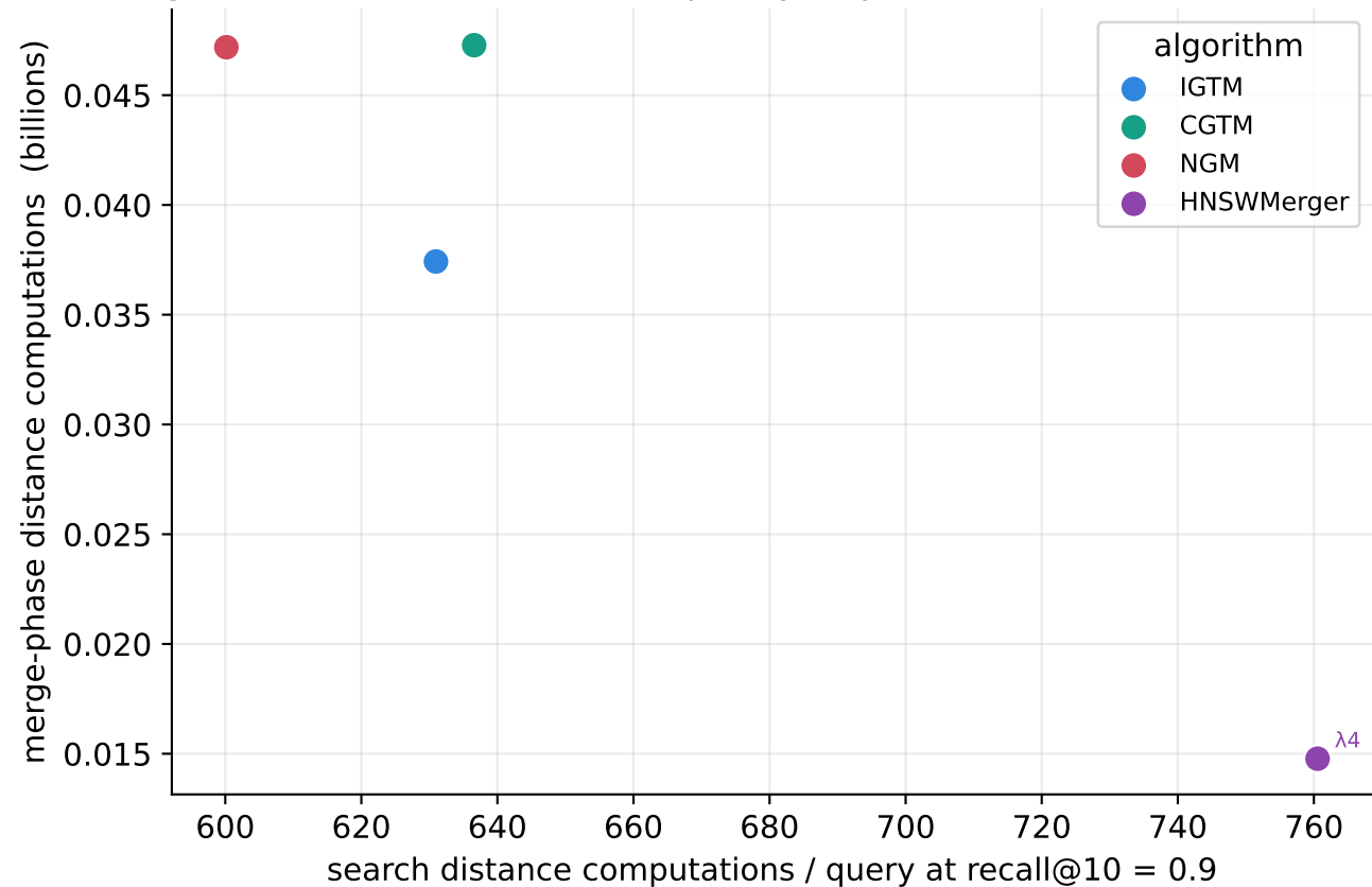
Merge cost at matched search quality, 2 partitions (SIFT 100K (BIGANN))
