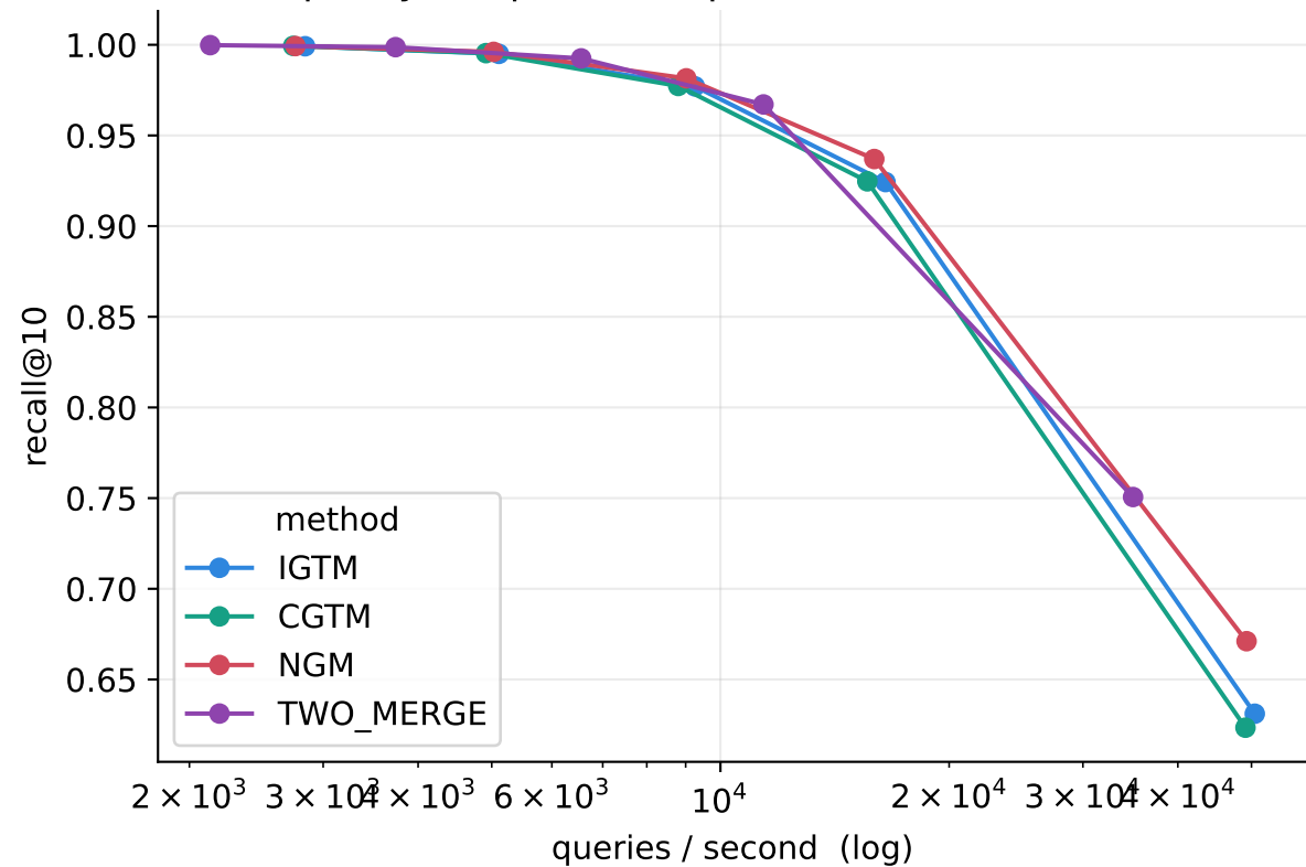
Search quality vs speed at 2 partitions (SIFT 100K (BIGANN))
