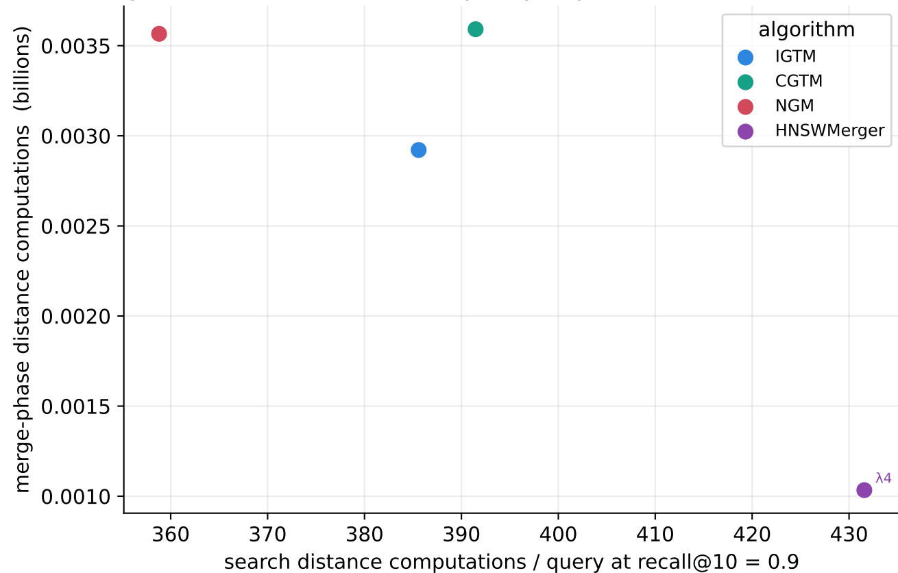
Merge cost at matched search quality, 2 partitions (SIFT 10K (BIGANN))
