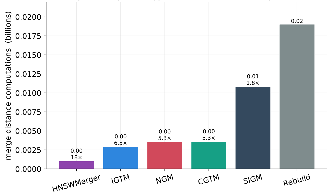
Merge cost by strategy (SIFT 10K (BIGANN), 2 partitions)
