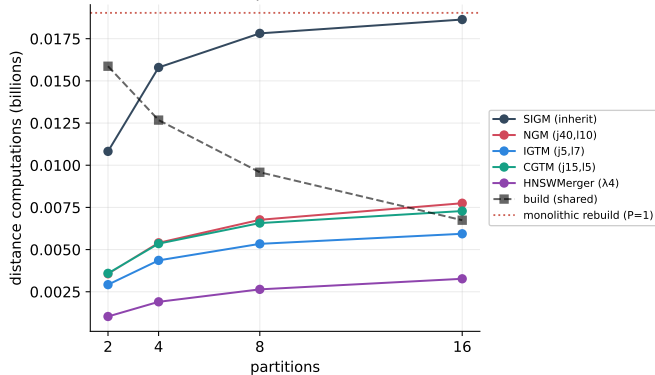
Divide-and-conquer trades more (parallelizable) build for more merge cost and slight recall loss (SIFT 10K (BIGANN)) Cost vs partition count
