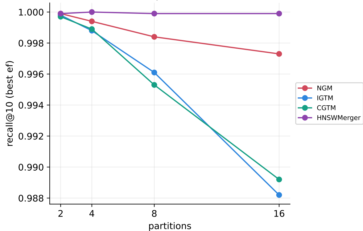
Recall vs partition count
