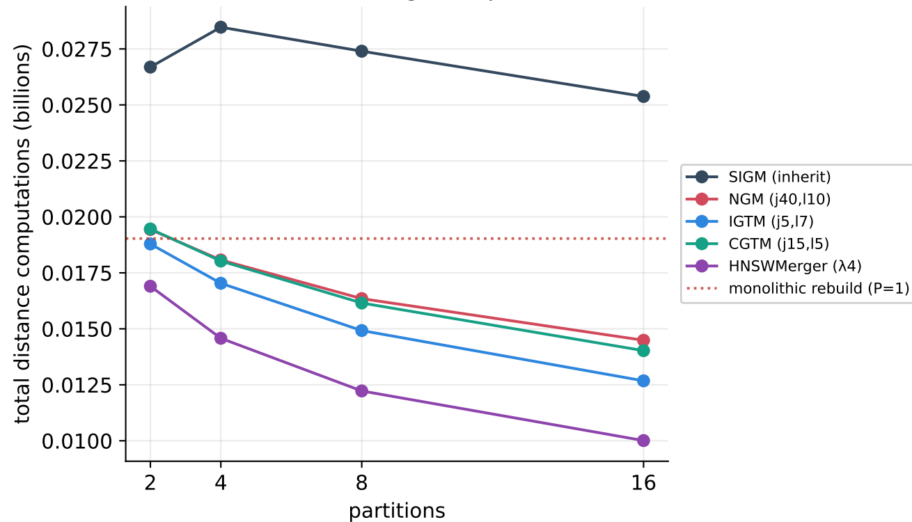
Total cost (build + merge) vs partition count
