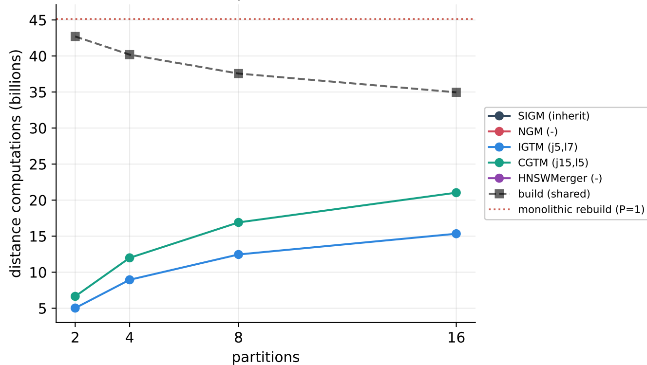
Divide-and-conquer trades more (parallelizable) build for more merge cost and slight recall loss (SIFT 10M (BIGANN)) Cost vs partition count
