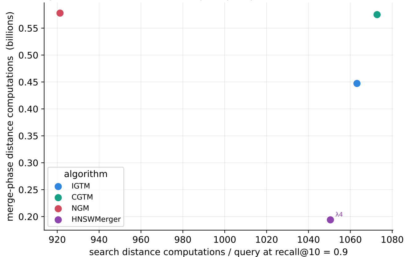
Merge cost at matched search quality, 2 partitions (SIFT 1M (BIGANN))
