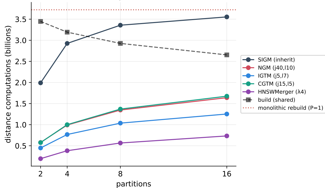
Divide-and-conquer trades more (parallelizable) build for more merge cost and slight recall loss (SIFT 1M (BIGANN)) Cost vs partition count
