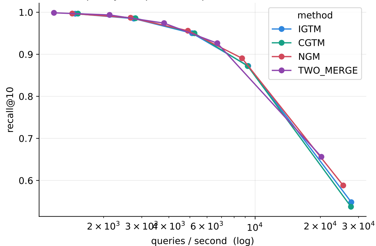
Search quality vs speed at 2 partitions (SIFT 1M (BIGANN))
