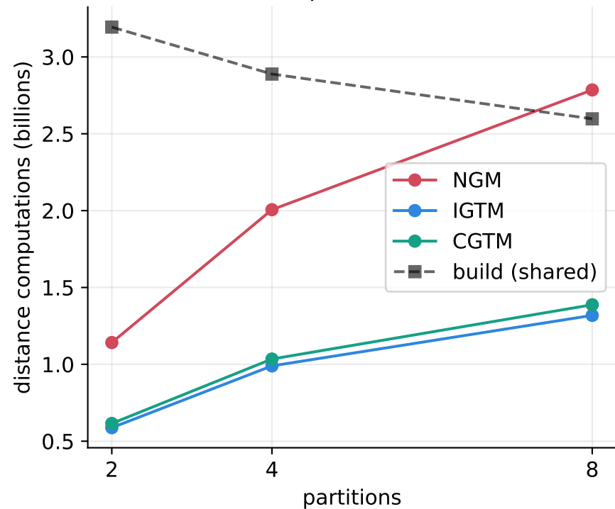
Divide-and-conquer trades more (parallelizable) build for more merge cost and slight recall loss Cost vs partition count
