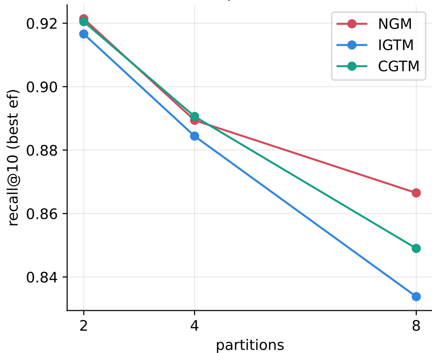
Divide-and-conquer trades more (parallelizable) build for more merge cost and slight recall loss (GIST1M) Cost vs partition count Recall vs partition count
