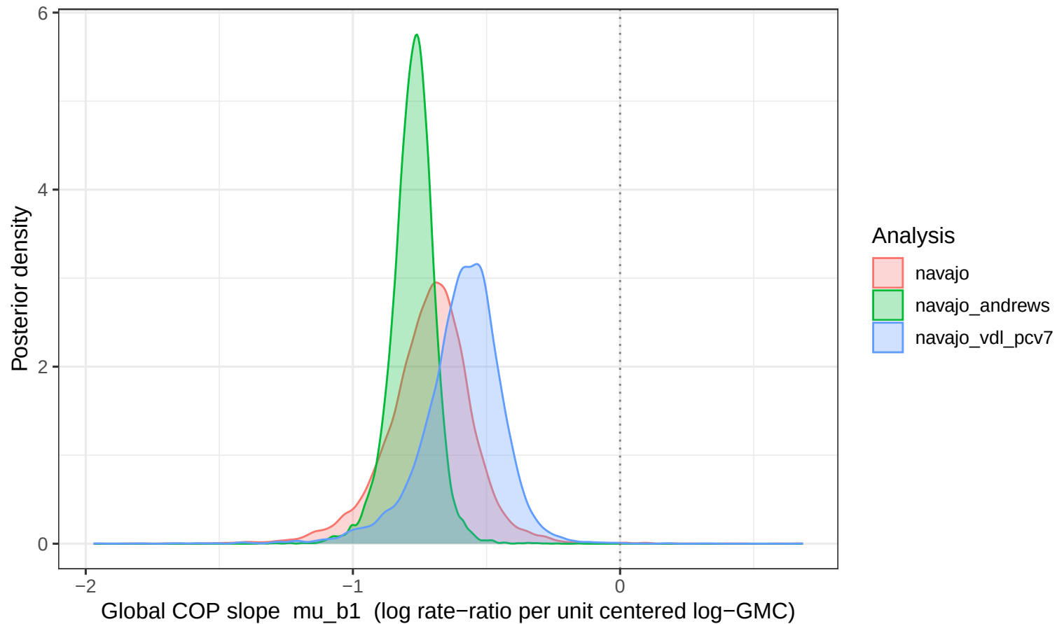
COP slope by outcome for Navajo immunogenicity (Whitney vs Andrews vs van der Lind
