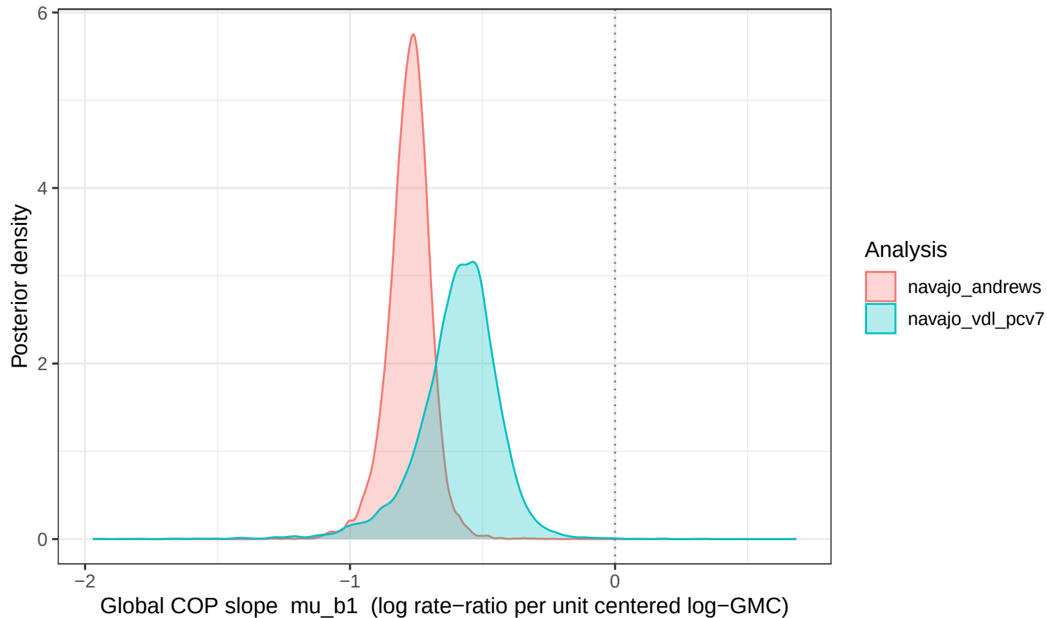
PCV7 COP slope by outcome for Navajo immunogenicity (Andrews vs van der Linden)
