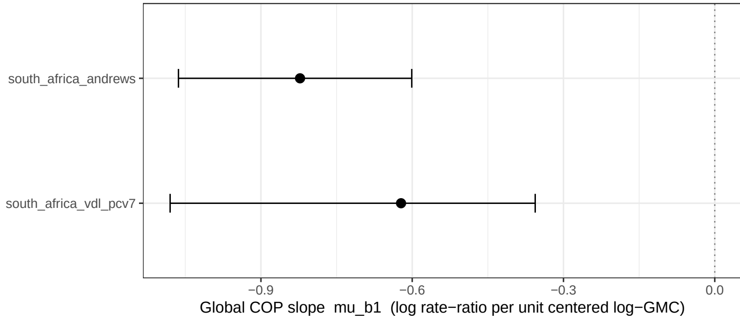
PCV7 COP slope by outcome for South Africa immunogenicity (Andrews vs Points = posterior median; bars = 95% credible interval
