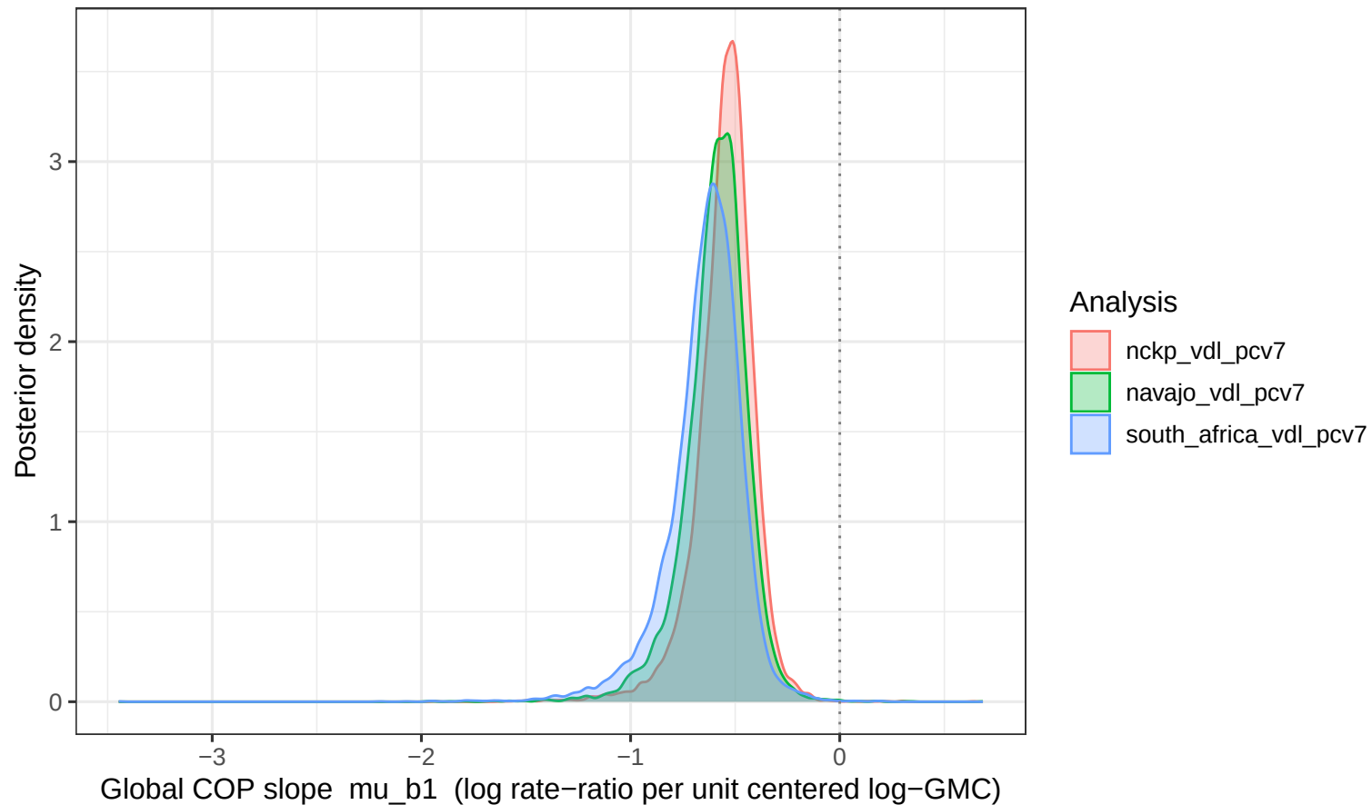
COP slope by immunogenicity source (outcome = van der Linden 2016 PCV7)
