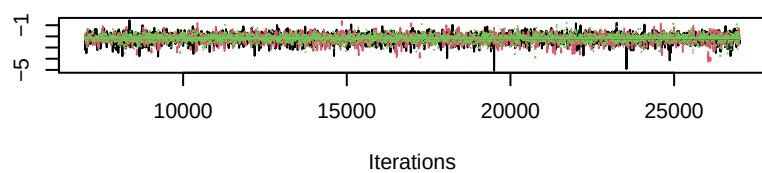
Trace of mu_a
