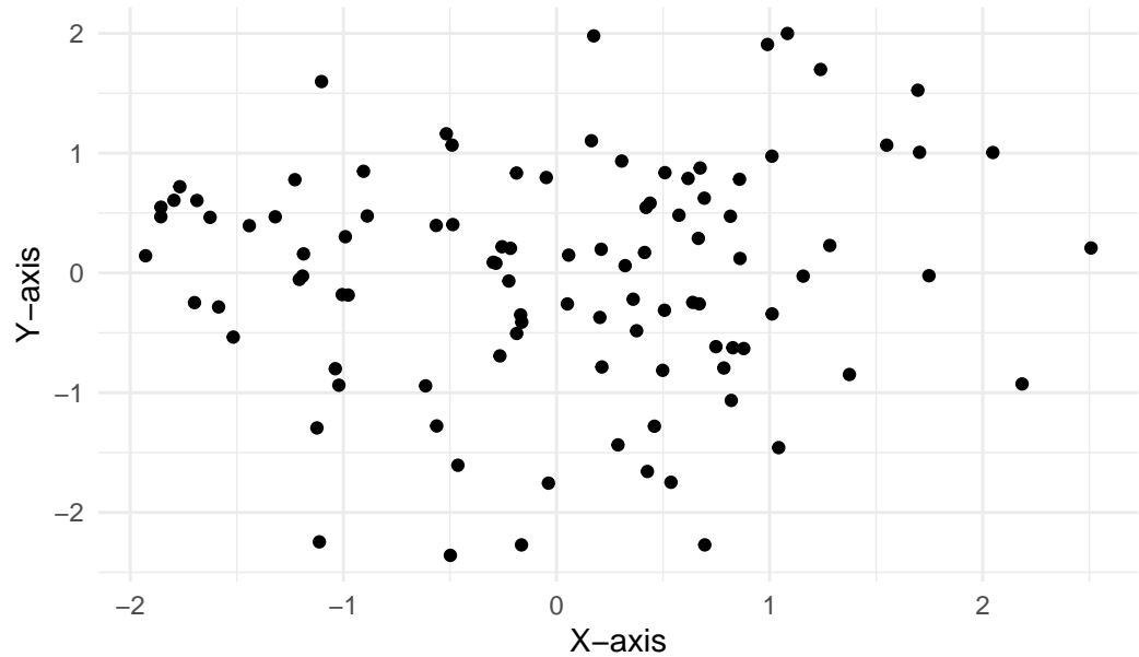
Scatter Plot of Sample Data
