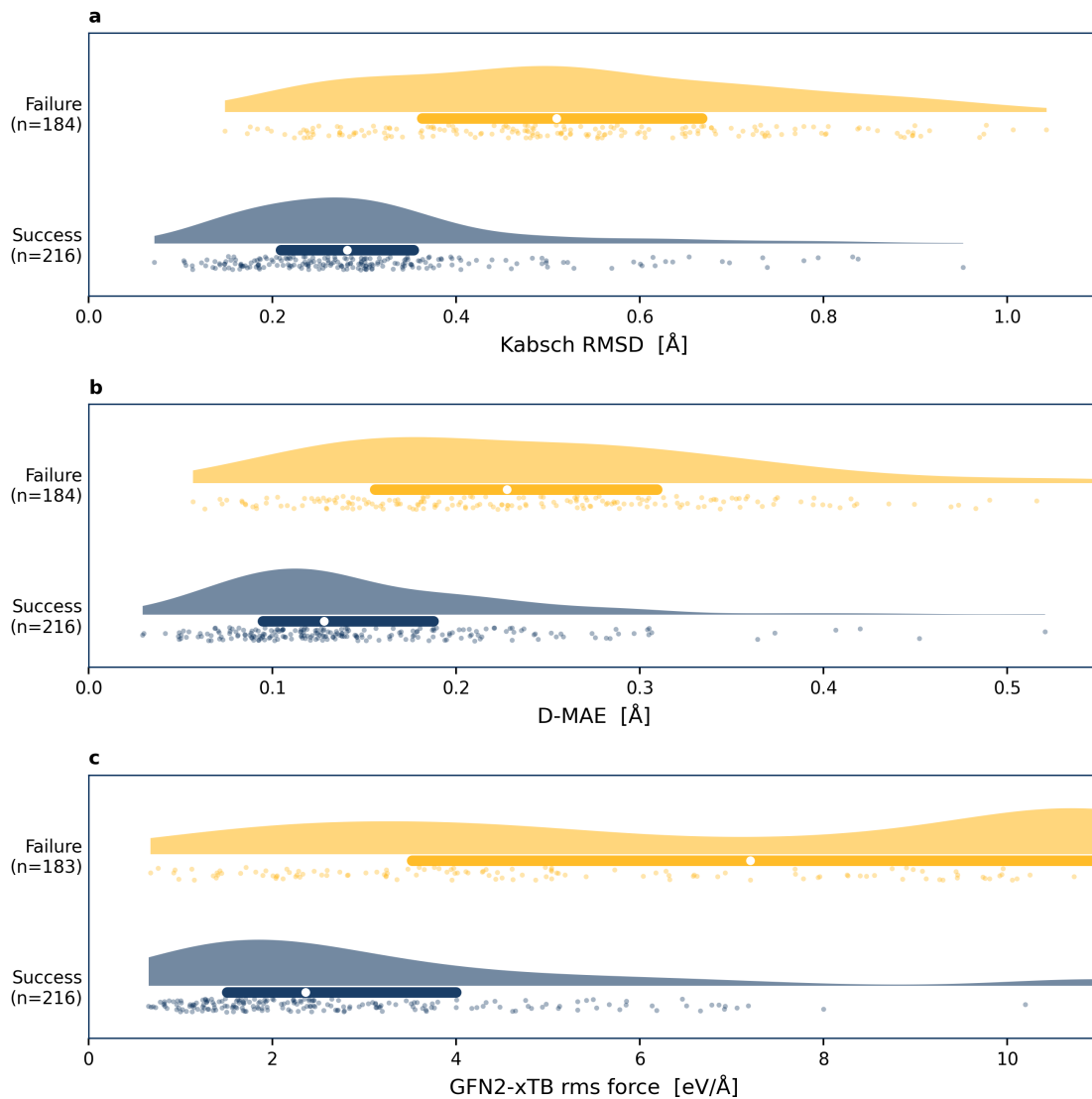
Figure 2: Rainclouds (half-violin, box with white median, and per-guess points) comparing the converged ( n = 216 ) and “failed” ( n = 184 ) classes for three representative guess-quality measures: (a) Kabsch RMSD, (b) D-MAE, and (c) the deployable GFN2-xTB rms force on the guess (failed n = 183 ). Class medians shift in the expected direction while the distributions overlap across most of their range.
