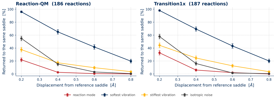
Figure 3: Return rates to the original saddle from controlled displacements (187 and 186 reactions, \sim 3200 trials per database). Points with the same displacement from the reference saddle differ only in the direction of that displacement, so the vertical spread is due to direction alone. Error bars are binomial standard errors.
