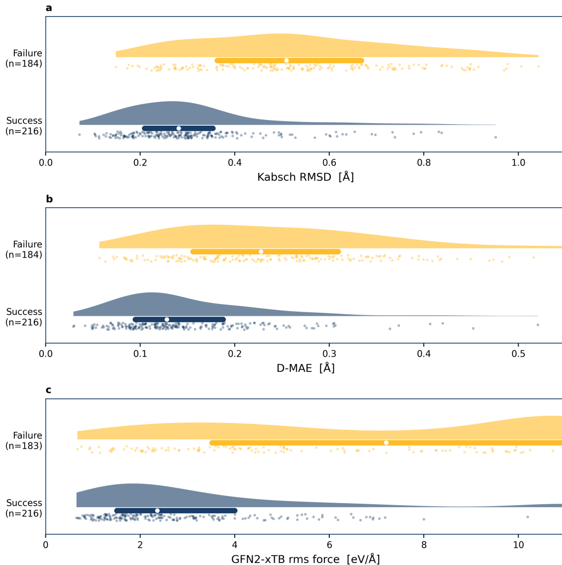
Figure 2: Guess-quality measures separate converged from failed optimizations only weakly. Rainclouds (half-violin, box with white median, and per-guess points) compare the converged ( n = 216 ) and “failed” ( n = 184 ) classes for three representative measures: (a) Kabsch RMSD, (b) D-MAE, and (c) the deployable GFN2-xTB rms force on the guess (failed n = 183 ). Class medians shift in the expected direction, but the distributions overlap heavily – low-metric guesses fail while high-metric guesses converge – so no fixed cutoff cleanly separates usable from unusable guesses.
