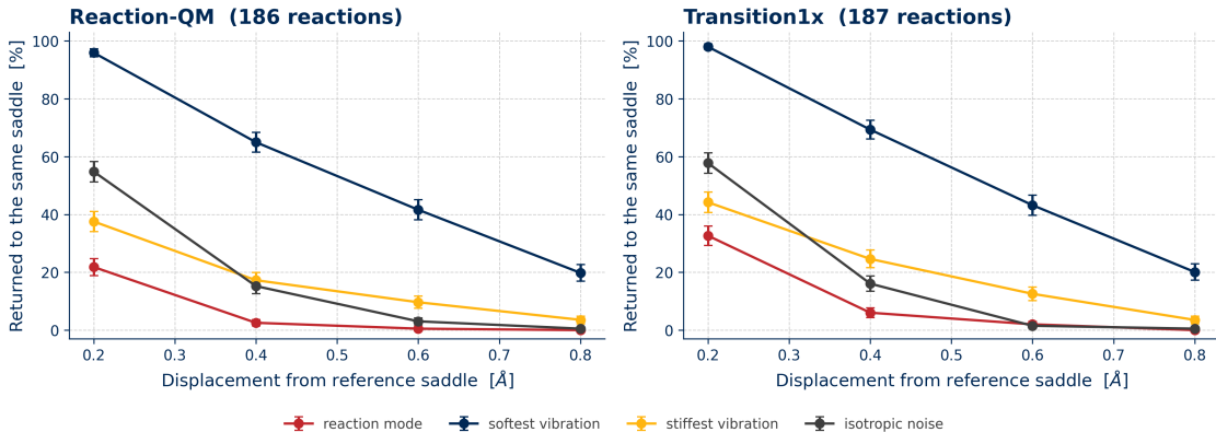
Figure 3: Controlled displacement from the reference saddle (187 and 186 reactions, \sim 3200 trials per database). Every point at a given abscissa sits at an identical distance from the saddle – verified to 10^{-3} Å for every trial – so the vertical spread is due to direction alone. Error bars are binomial standard errors.
