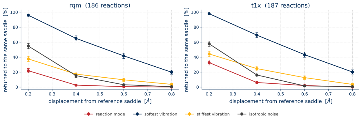
Figure 3: Controlled displacement from the reference saddle (187 and 186 reactions, \sim 3\,200 trials per database). Every point at a given abscissa sits at an identical distance from the saddle — verified to 10^{-5} Å for every trial — so the vertical spread is due to direction alone. Error bars are binomial standard errors.
