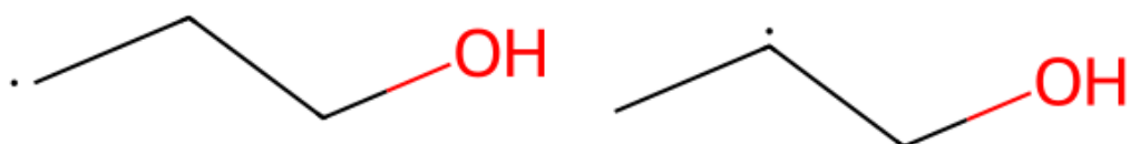
Radical-site migration
