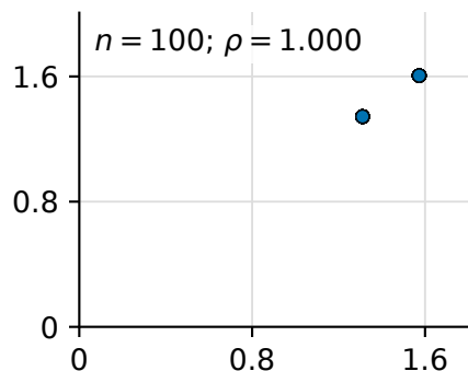
5-point stencil
