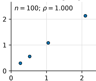
Embedding bag
