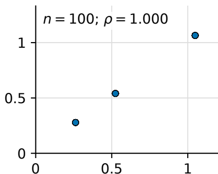
Embedding bag
