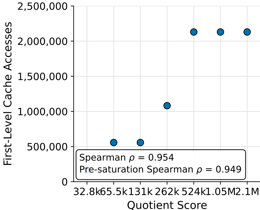
Quotient Score versus First-level Cache Accesses for EMBEDDING BAG Kernel
