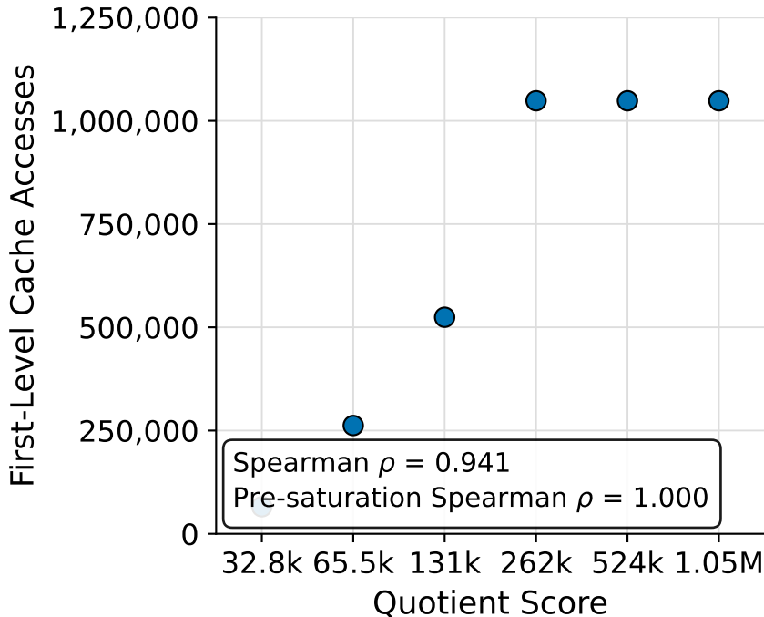
Quotient Score versus First-level Cache Accesses for GEMV Kernel
