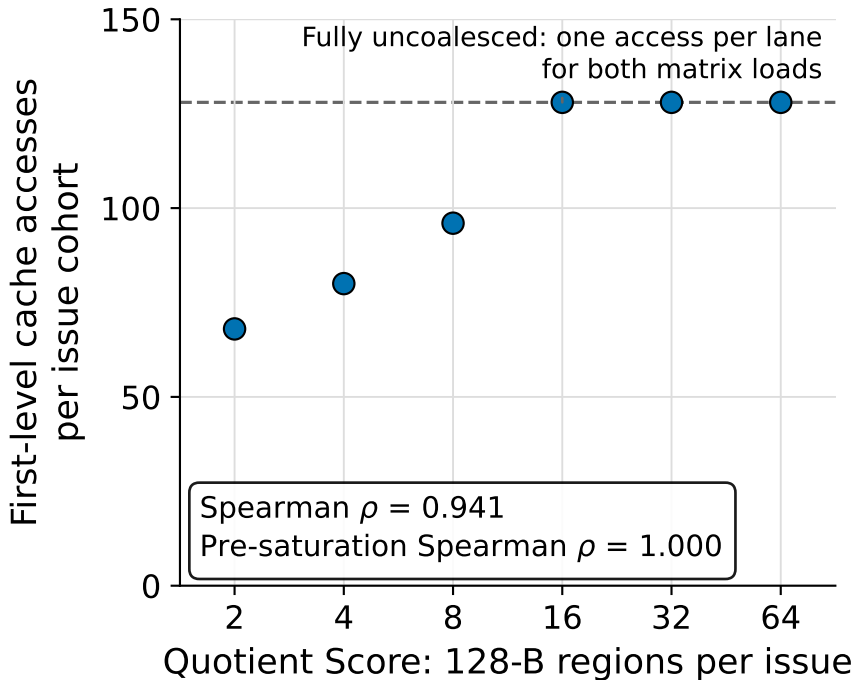
Quotient Score versus First-level Cache Accesses for GESUMMV Kernel
