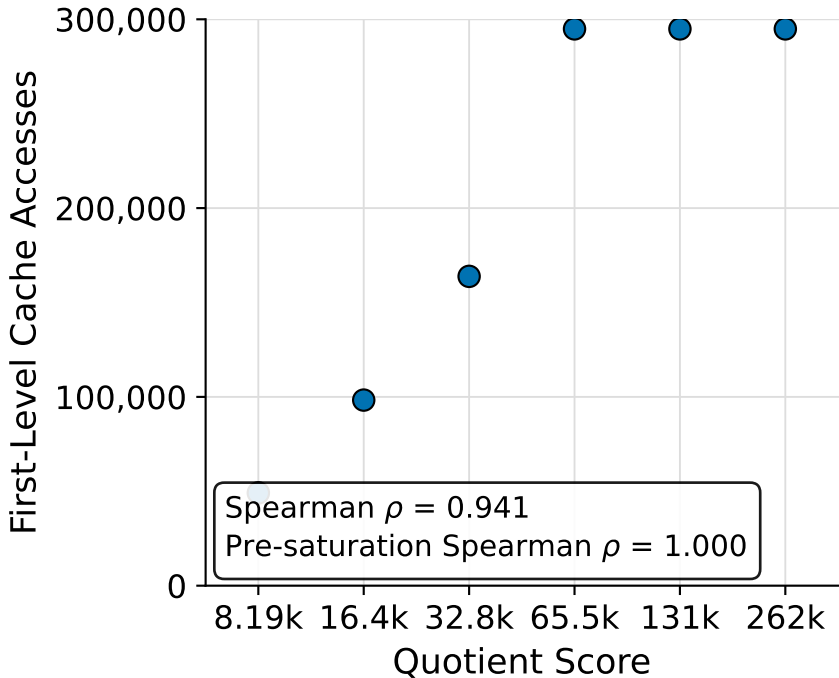
Quotient Score versus First-level Cache Accesses for SOFTMAX BIAS Kernel
