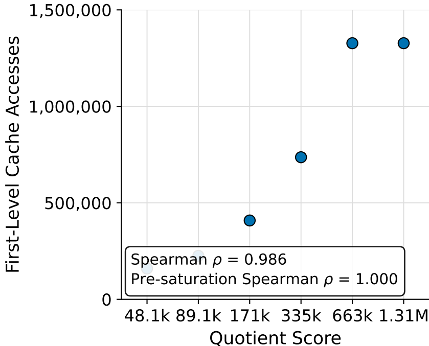
Quotient Score versus First-level Cache Accesses for STENCIL5 Kernel
