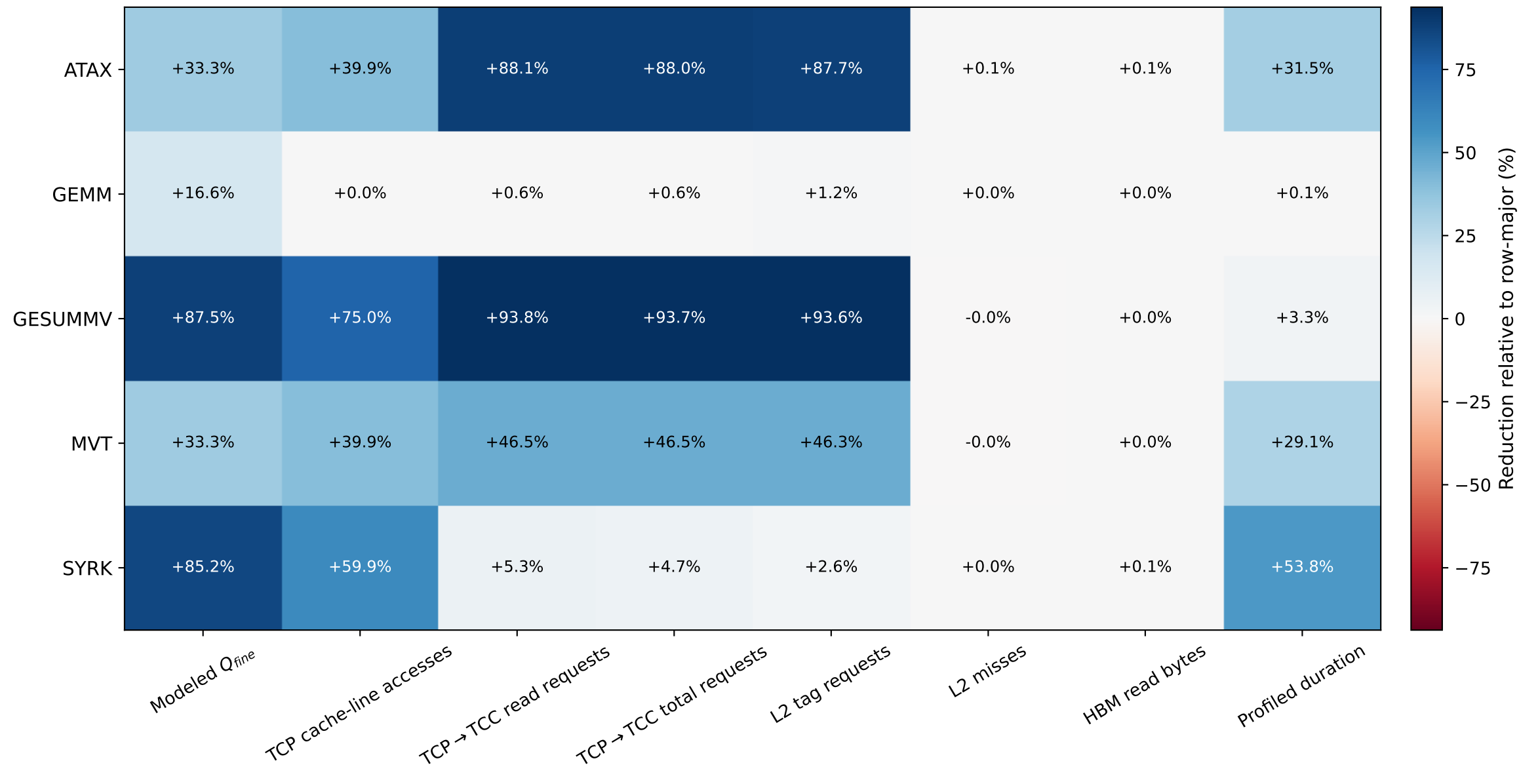
LAQS-selected versus row-major: positive values mean fewer requests
