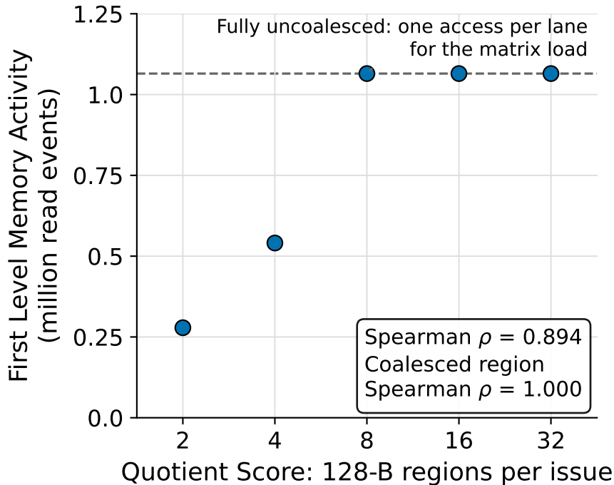
Quotient Score versus First Level Memory Activity (read events) for GEMV Kernel on NVIDIA H100
