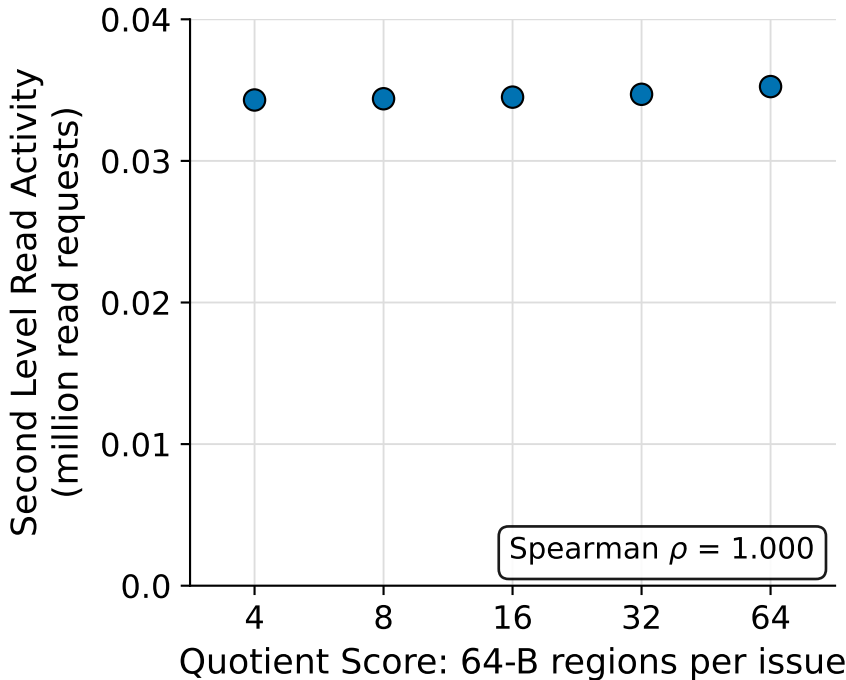
Quotient Score versus Second Level Read Activity for GEMV Kernel on AMD MI300A
