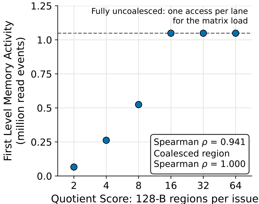
Quotient Score versus First Level Memory Activity (read events) for GEMV Kernel on AMD MI300A
