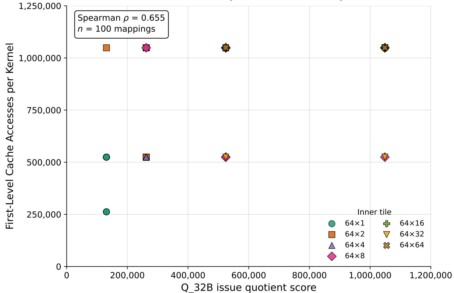
GEMV: random tile layouts versus memory traffic
